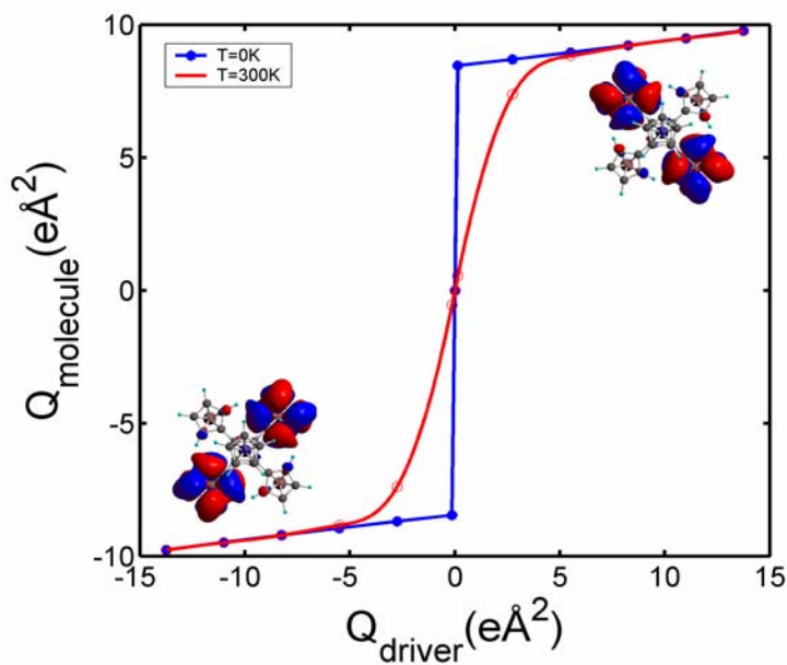
Figure 2: The response function of \{\eta^5\text{-C}_5\text{H}_5\}\text{Fe}(\eta^5\text{-C}_5\text{H}_4)_4(\eta^4\text{-C}_4)\text{Co}(\eta^5\text{-C}_5\text{H}_5) dication when driven by a quadrupole driver. For each driver quadrupole moment the induced molecular quadrupole moment is calculated. Blue ( T = 0 K). Red ( T = 300 K).
