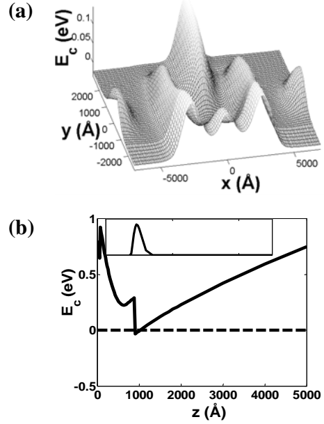
Figure 2: Potential energy profile (a) in the xy plane at the 2DEG interface (b) along the z direction with the inset showing the ground state wavefunction under bias condition V_L=V_R=V_{QPC-L}=V_{QPC-R}=V_M=V_T=-0.585 V, V_{PL}=V_{PR}=-0.15 V.
