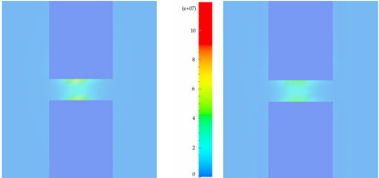
Figure 1. One cutplane along the axis of the channel of the 3-D test structure shows the anion (Cl - ) density for a situation with positive fixed charge on the “channel” walls at equilibrium. Left picture shows the result from traditional PNP theory. Right side picture shows the result from modified PNP theory with ECP correction. The scale in the colorbar is: (6.022e6=1000mM/L).
